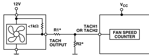
Figure 9d. Fan with Strong Tach. Pull-Up to >V_{CC} or Totem-Pole Output, Attenuated with R_1/R_2
