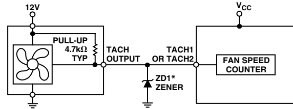
Figure 9b. Fan with Tach. Pull-Up to Voltage >6.5 V (e.g., 12 V) Clamped with Zener Diode
