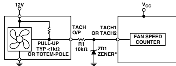
Figure 9c. Fan with Strong Tach. Pull-Up to >V_{CC} or Totem-Pole Output, Clamped with Zener and Resistor
